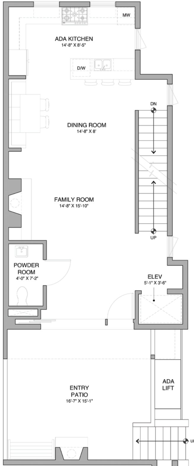
First Floor
